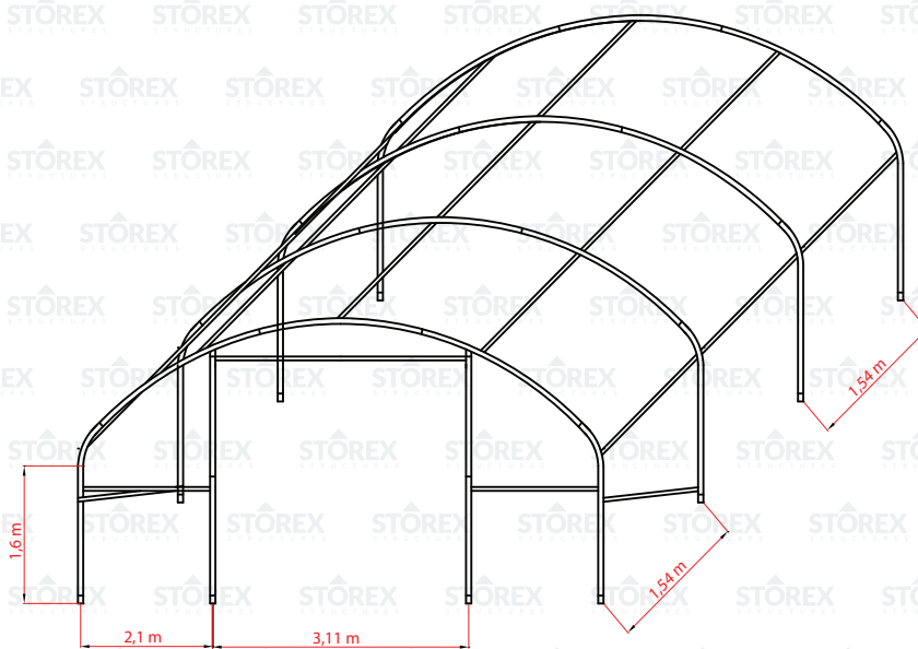
Partial 3D drawing (not all frame arches are shown)
